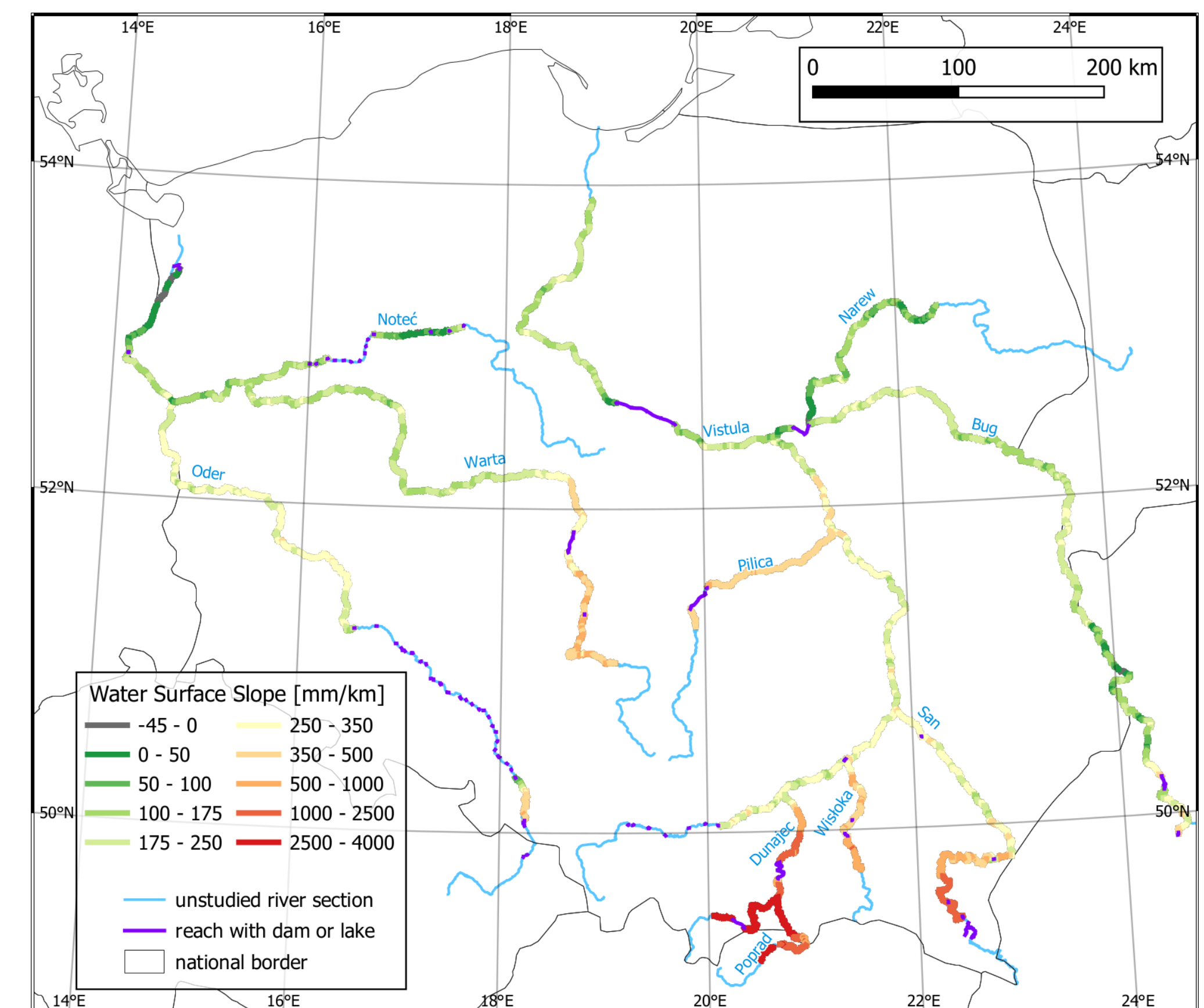
Fig. 6. Water Surface Slope of the 11 investigated Polish rivers.
