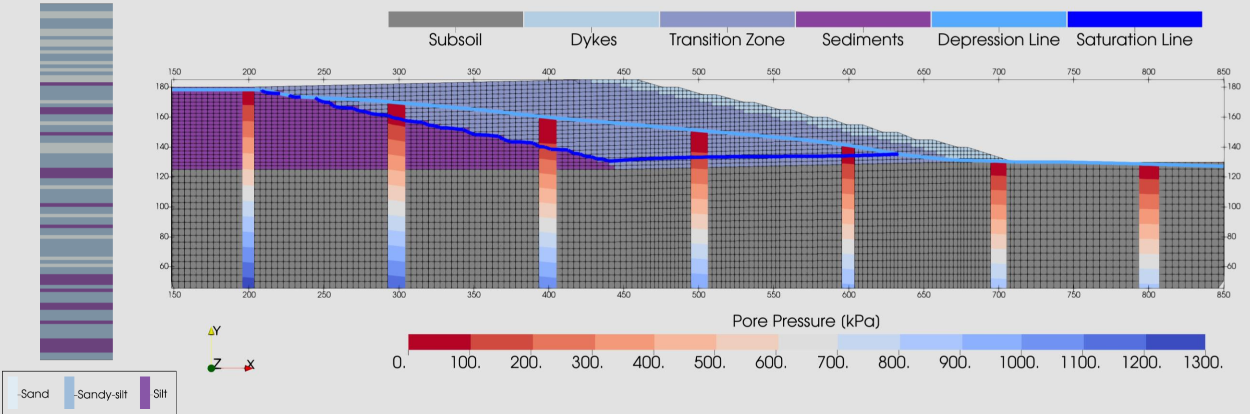
Tailing Profile
